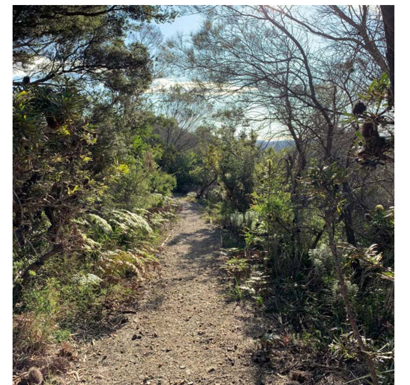
CUT AND BENCHED TRACK
